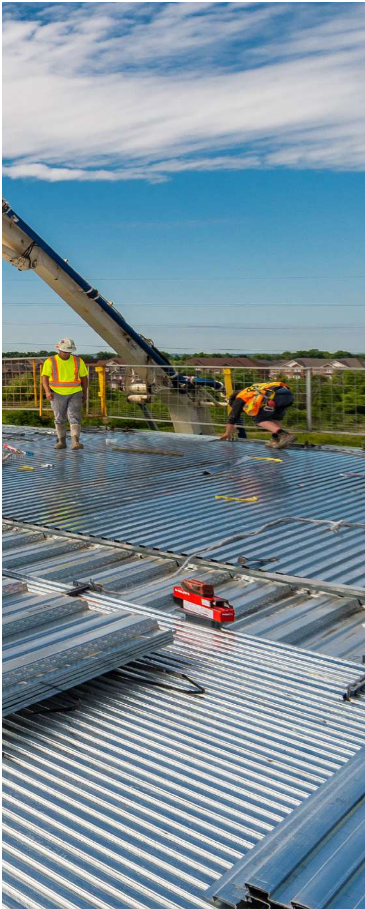
Construction at Trend Living, Waterdown; one of the 12 NHDG buildings constructed with geothermal energy
